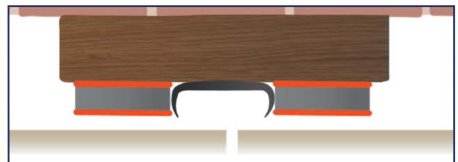
SCHEMATIC CROSS SECTION (TOP VIEW) BOSTIK PAD-SYSTEM:
